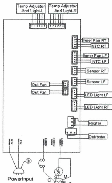
Electrocircuit Line Diagram
