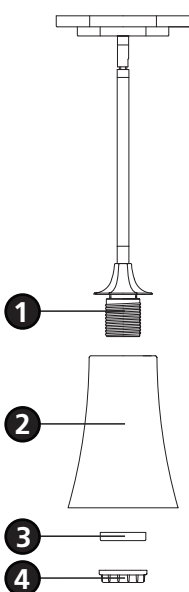
Drawing 3 - Glass Installation
