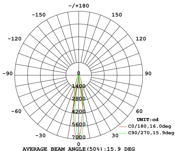
20° Beam Angle - 120V Input
