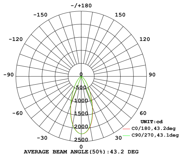
45° Beam Angle - 120V Input
