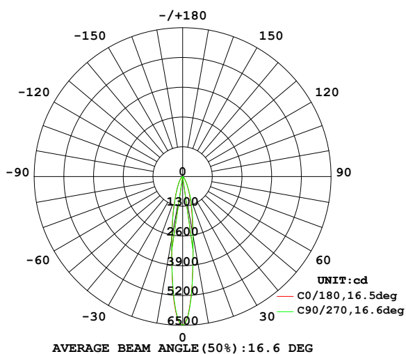
20° Beam Angle - 277V Input
