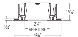
EDL-2000 Series
