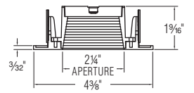
EDL-2100 Series
