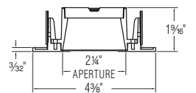
EDL-2200
