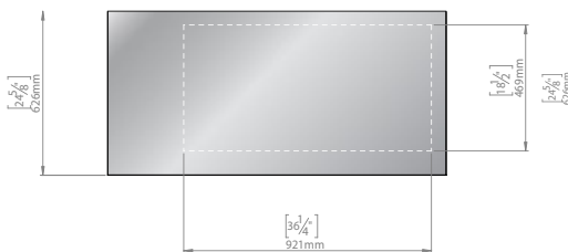
FBB-24-48 Front View
