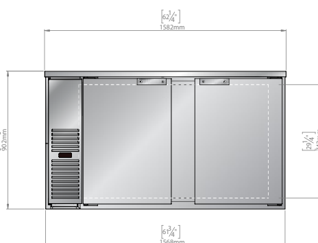
FBB-24-60 Front View
