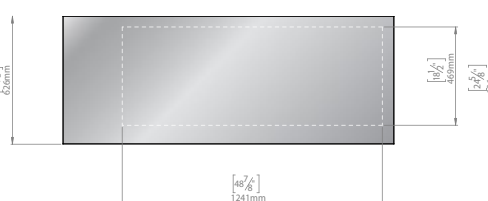
FBB-24-60 Front View
