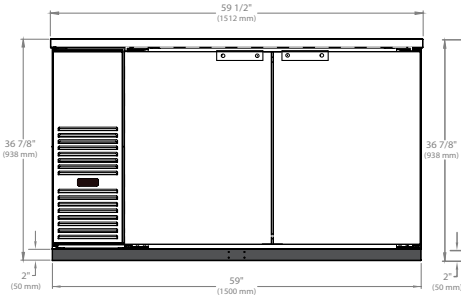
FBB-59(S) Front View
