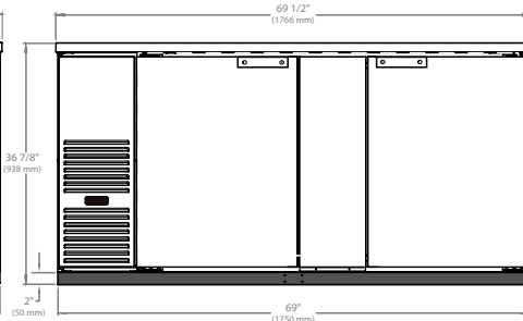
FBB-69(S) Front View
