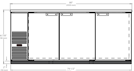
FBB-79(S) Front View
