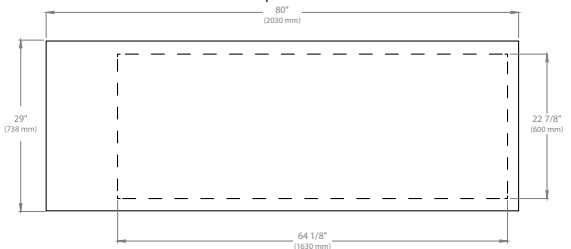
FBB-79(S) Top View
