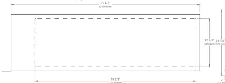
FBB-95 (S) Front View
