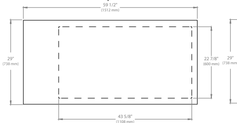
FBB-59(S) Top View
