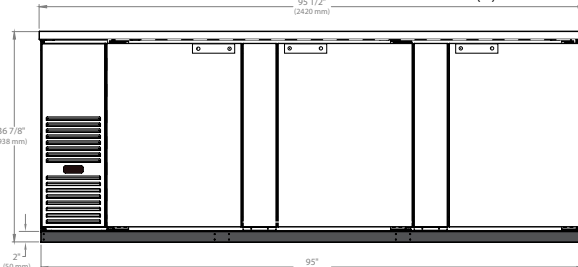
FBB-95(S) Front View
