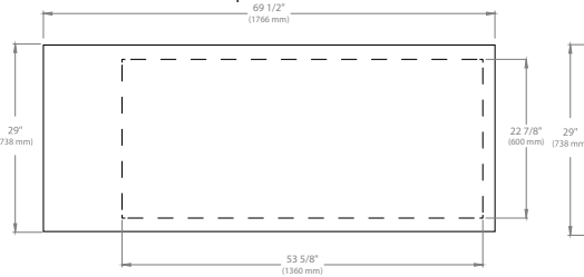
FBB-69(S) Top View
