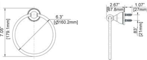
Towel Ring SA-1104
