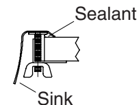
Self-Rimming Installation
