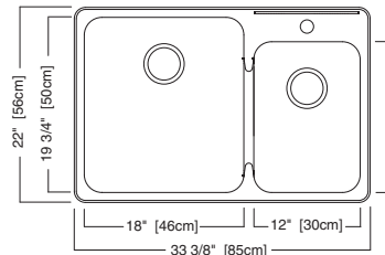
15CR.332911.073 Optional drilling: 1 hole on center
