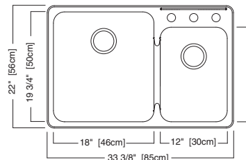
15CR.332983.073 Standard drilling: 3 hole
