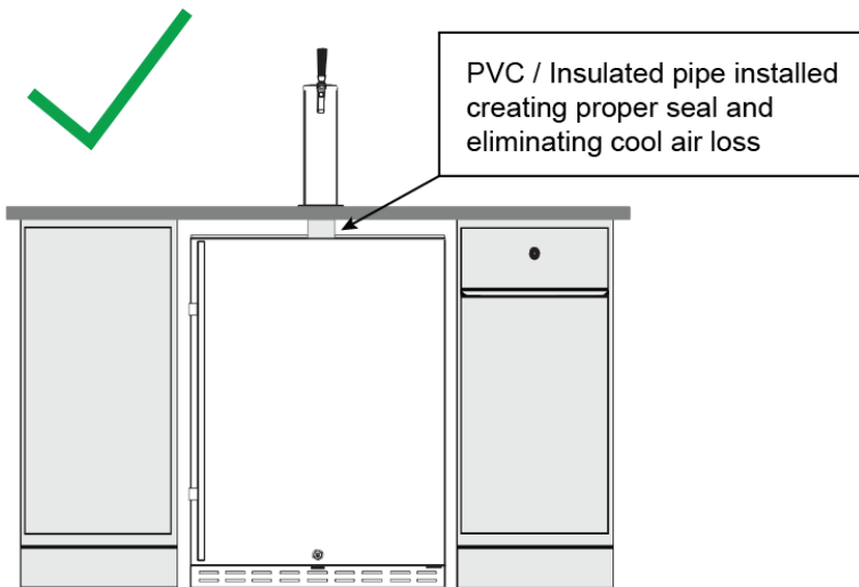
Correct Installation
