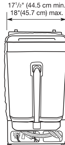
REAR VIEW
