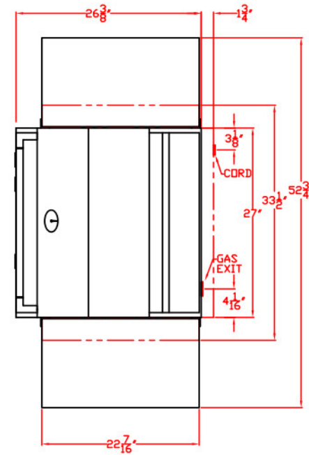
TOP VIEW
