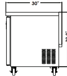
Side View of all Undercounter Units
