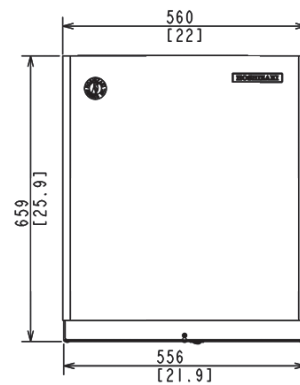
REMOTE AIR-COOLED
