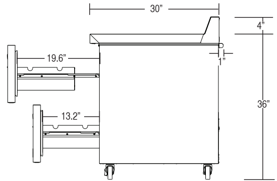
CRMR72-WD6 SIDE VIEW
