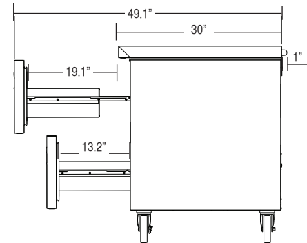
CRMR60-D4 SIDE VIEW
