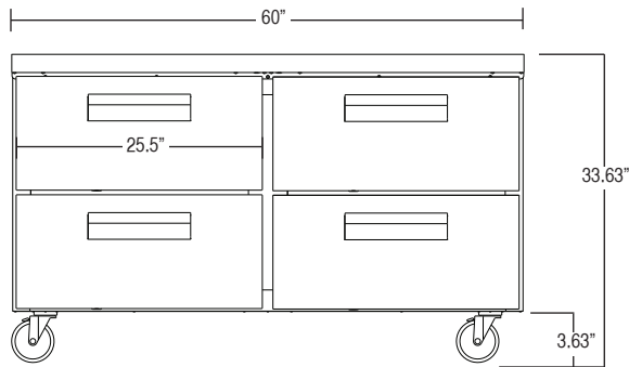
CRMR60-D4 FRONT
