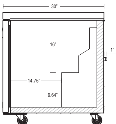
CRMF27-LP SIDE VIEW (Cross Section)
