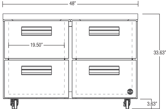
CRMF48-D4 FRONT
