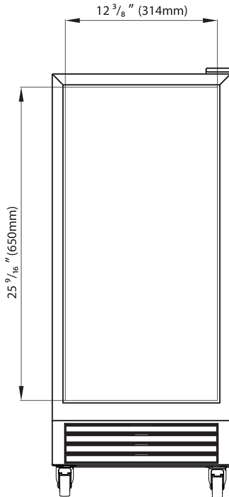
Front View
