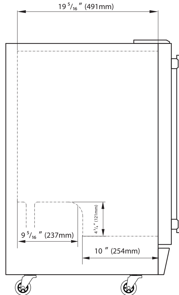
Side View
