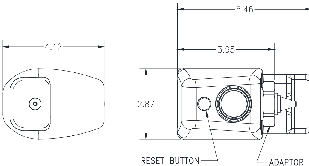
Rough-in dimensions/Overview dimensions
