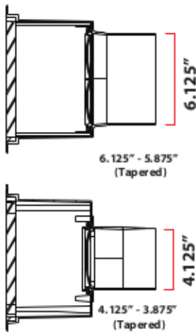
SECTIONAL VIEWS
