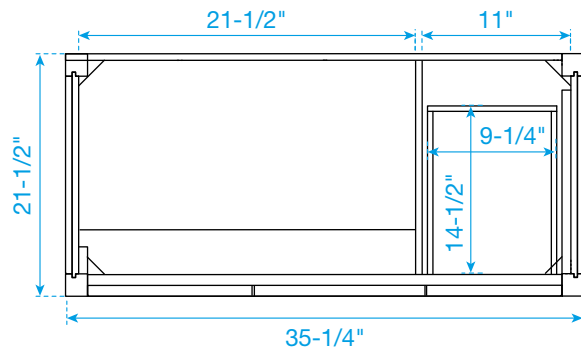
TOP VIEW OF VANITY CABINET
