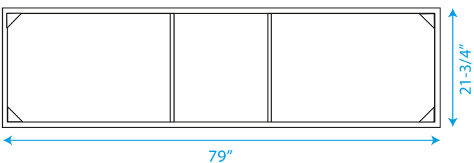
TOP VIEW OF VANITY CABINET
