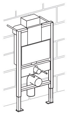
Pre-wall installation, top or front activation.
