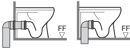
A. Floor-Mount Rear Discharge into Wall
