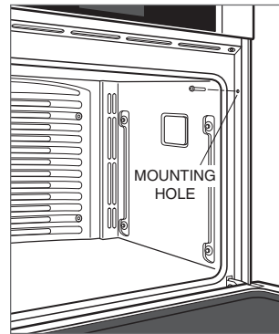
Hole location.
