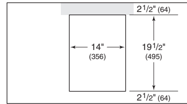
COUNTERTOP CUT-OUT
