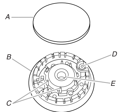
A. Burner cap B. Burner base C. Alignment pins D. Igniter E. Gas tube opening
