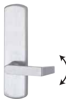
Lever or knob always active. Use BE suffix, e.g., 996L-BE. (Passage)
