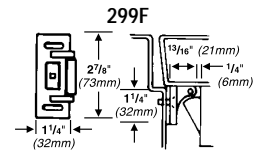
Projection 13/16" (21mm)
