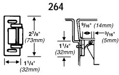
Projection 9/16" (14mm)
