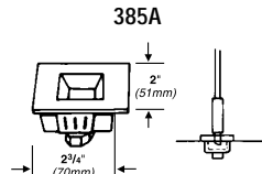
Mortise 2-1/2" (64mm)
