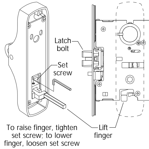
Figure 4. Adjust Lift Finger
