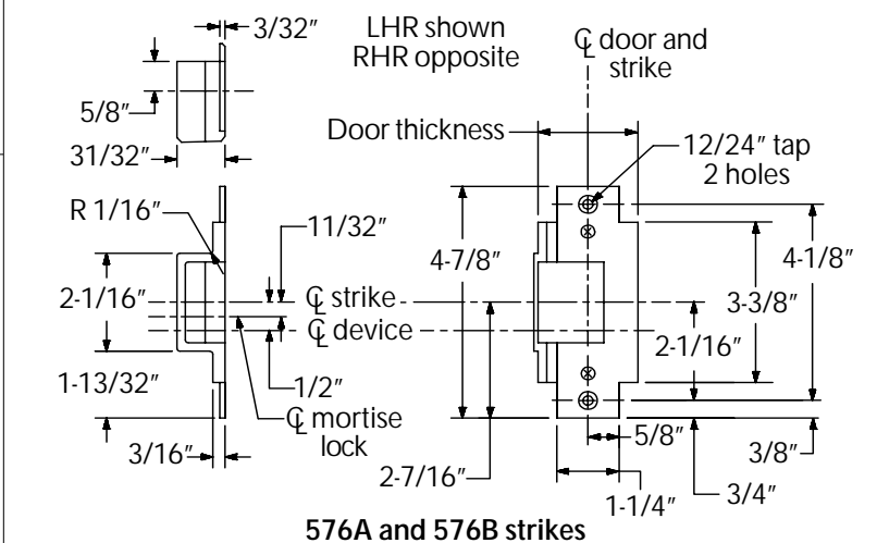
Figure 5. Prepare Frame for Strike
