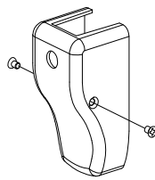
8827-F Top Latch Cover Kit Part No. 050465
