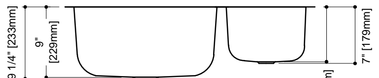
VISTA FRONTAL
