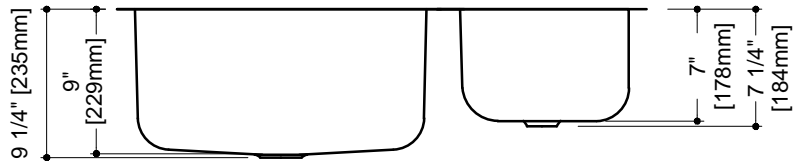
FRONT VIEW
