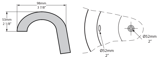
Rim detail
