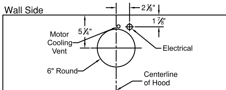
CONNECTION DIAGRAM
