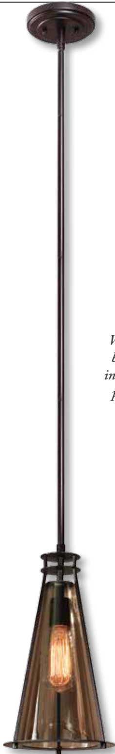
21965 Frisco, 1 Lt. Mini Pendant 14"H x 8" Dia. Includes: 1-40 watt ST64 bulb Adjustable Heights 24", 30", 36", 42", 48", 54" 60" 1-100 watt max, Edison Socket
