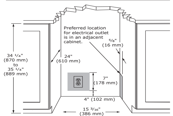
Cabinet Cut-Out
