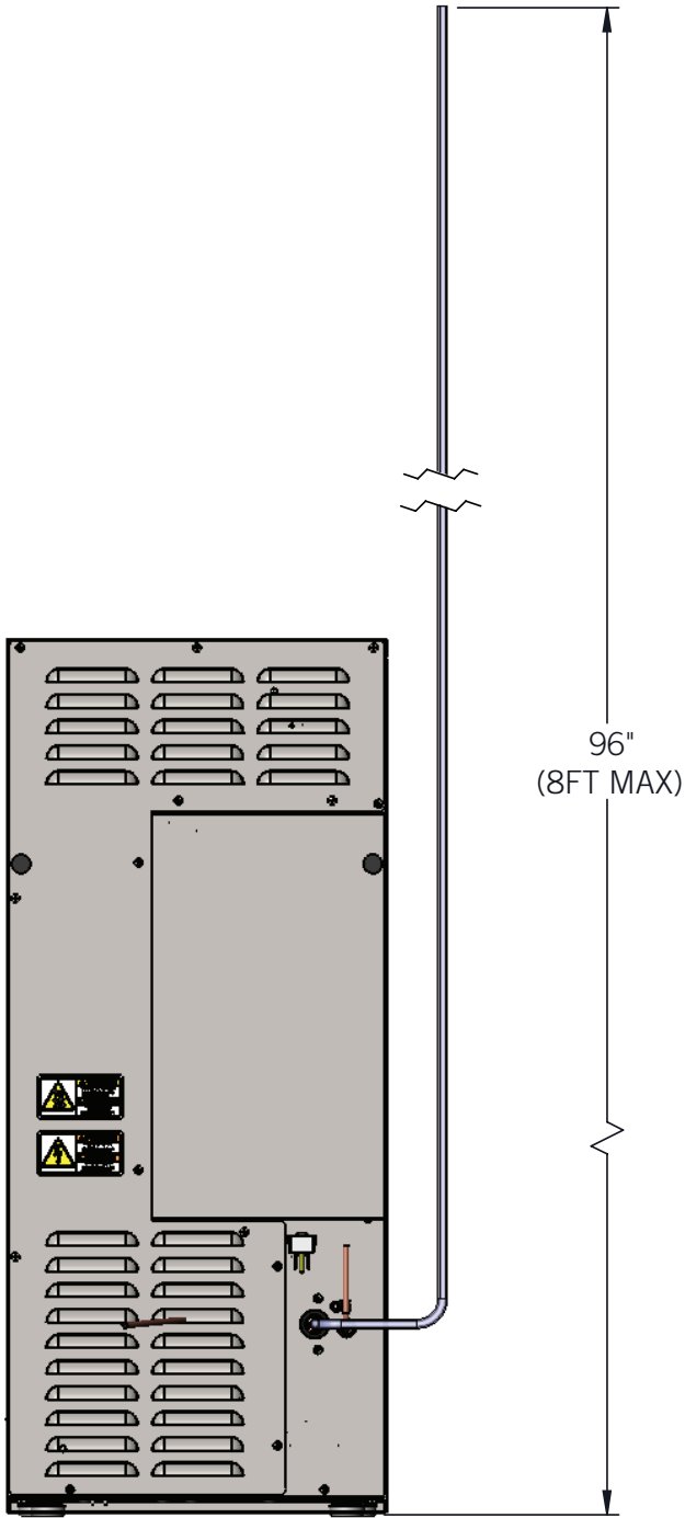
STANDARD PUMP WITH 3/8" O.D. HOSE
