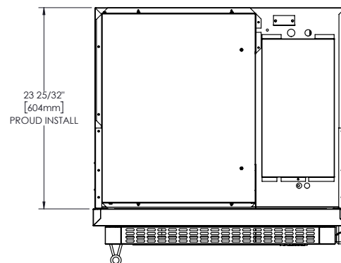
TOP VIEW FIGURE 3 - PROUD INSTALL
