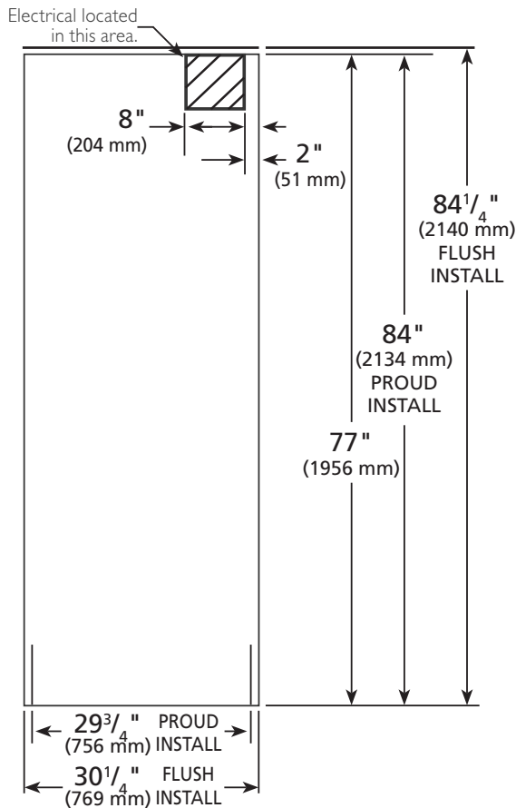
FRONT VIEW FIGURE 1 - ROUGH OPENING & ELECTRICAL AREA
