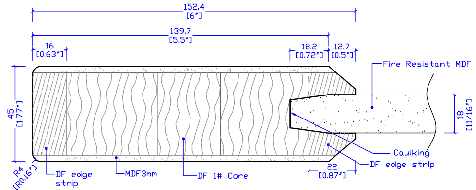
1800FR SECTION A-A
