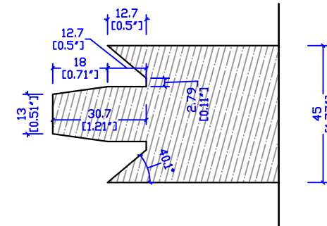
1800FR RAIL SECTION
