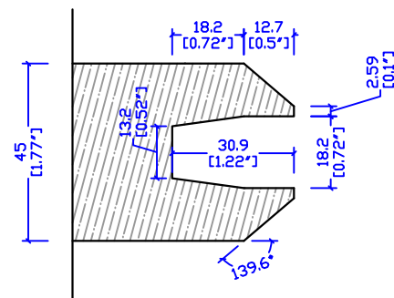
1800FR STILE SECTION
