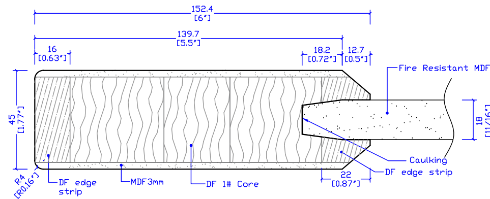
1800FR SECTION A-A
