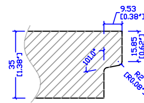
RAIL SECTION
