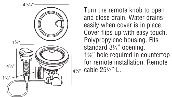
2310 Remote Covered Flip Top Sink Strainer.
