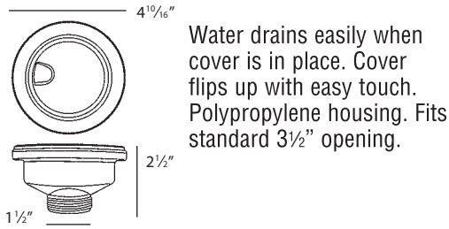
2210R Covered Flip Top Sink Strainer.
