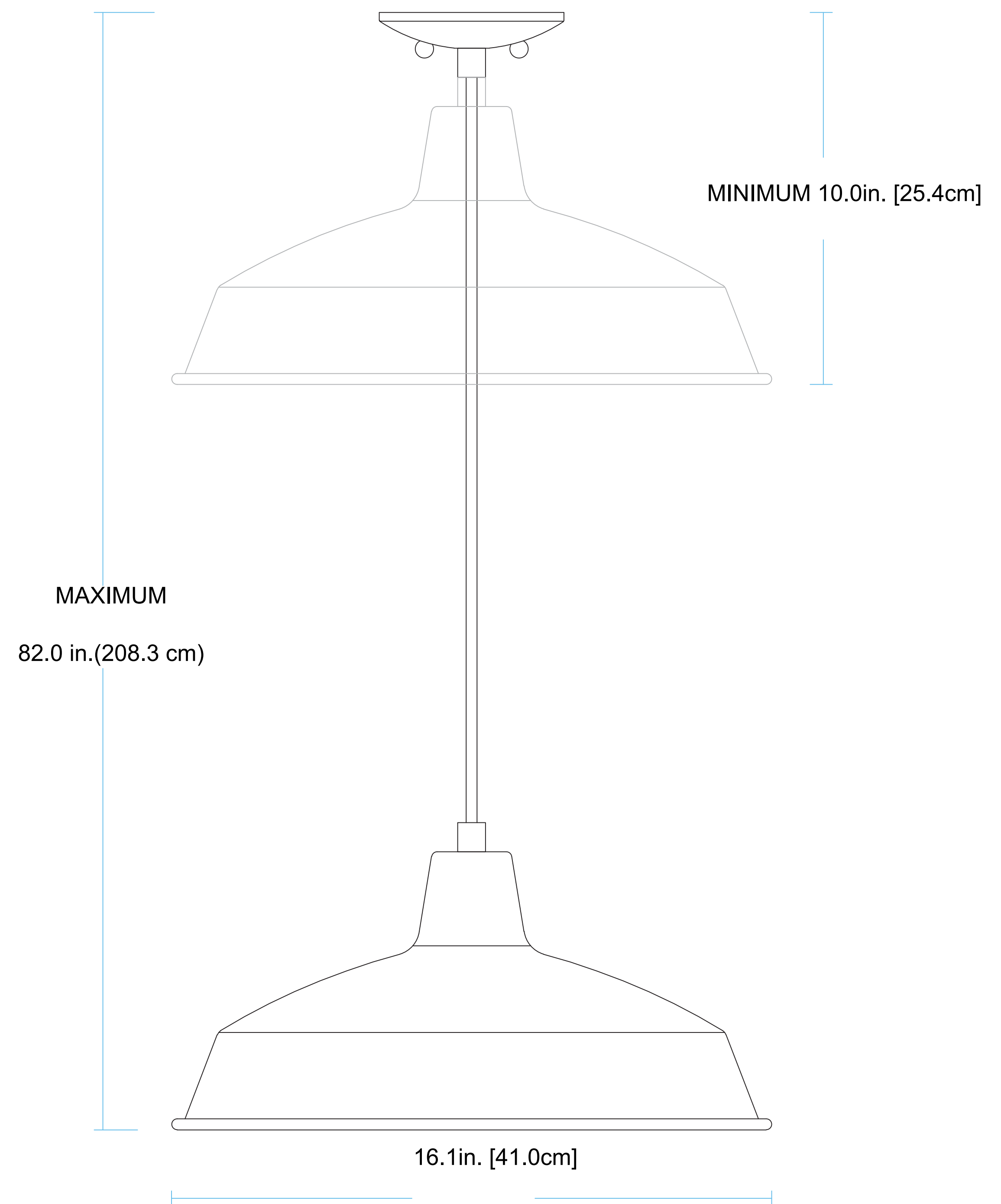
SIDE VIEW
