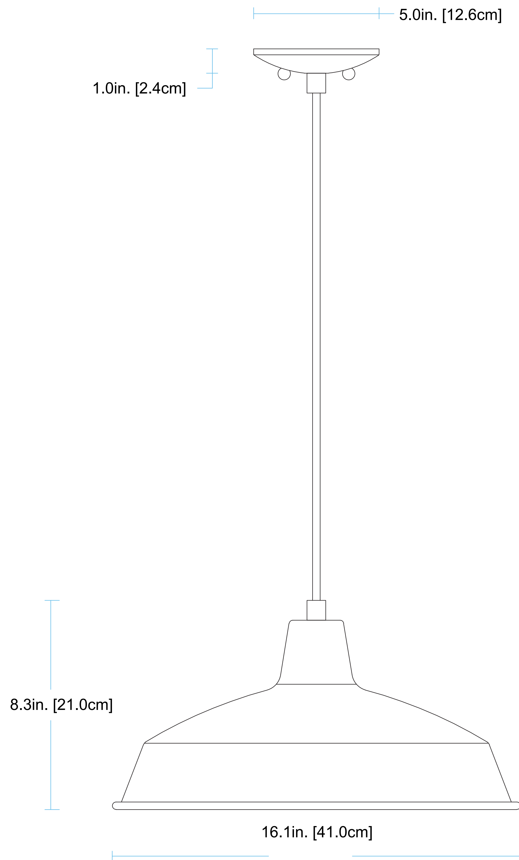
FRONT VIEW
