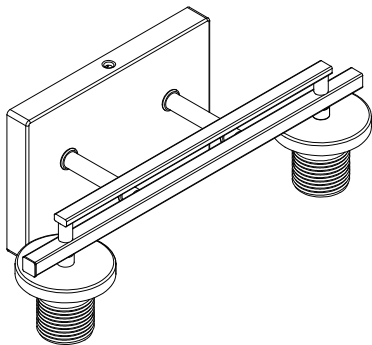
Fixture
