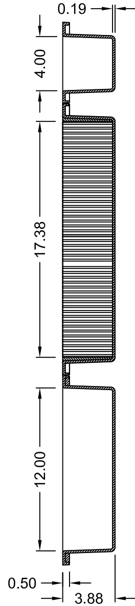
SECTION C-C
