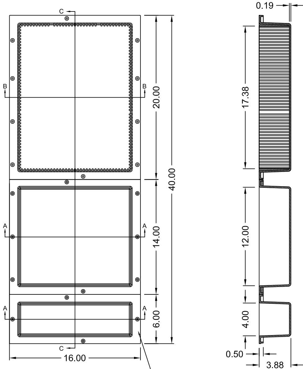
SECTION C-C
