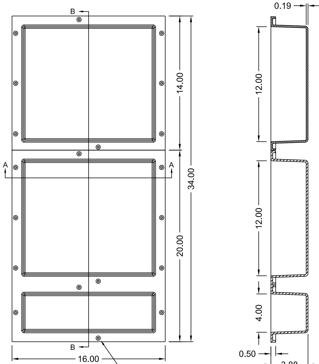
SECTION B-B
