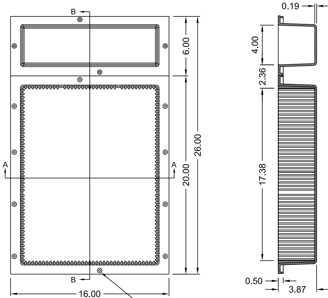
SECTION B-B
