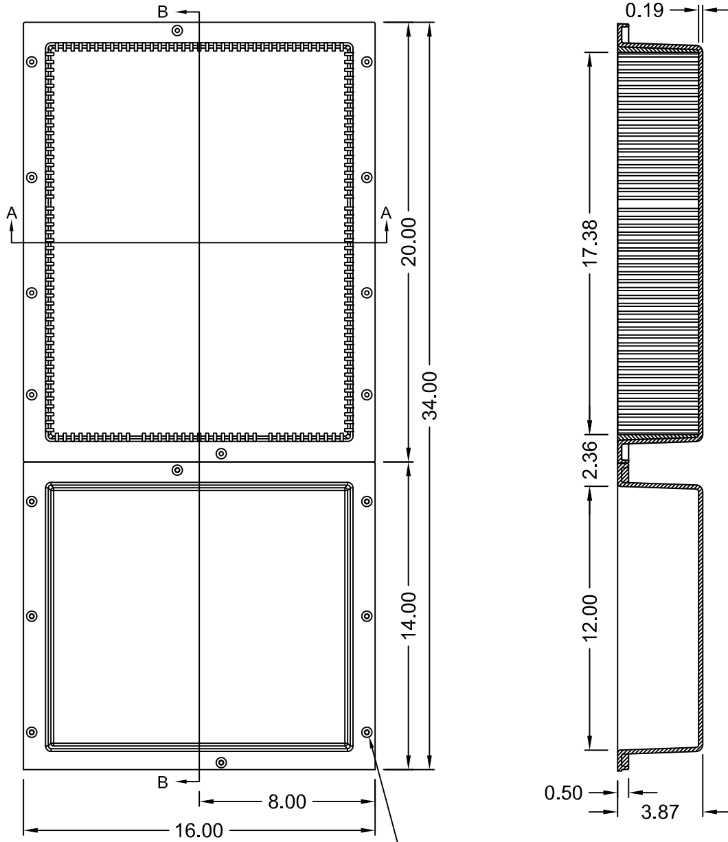
SECTION B-B
